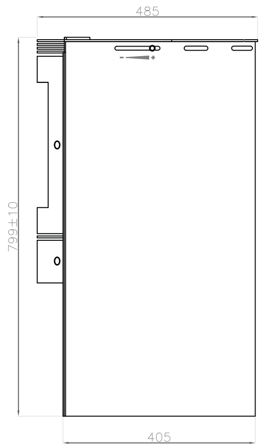
SIDE VIEW
